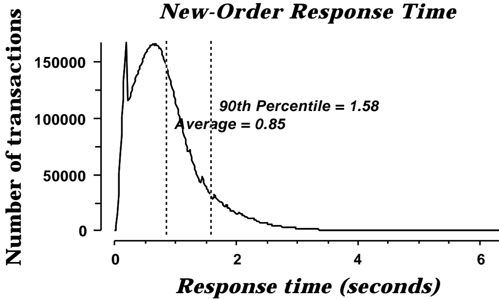
Figure 6-3-1. IBM eServer pSeries 660 Model 6M1 New-Order Response Time Distribution
