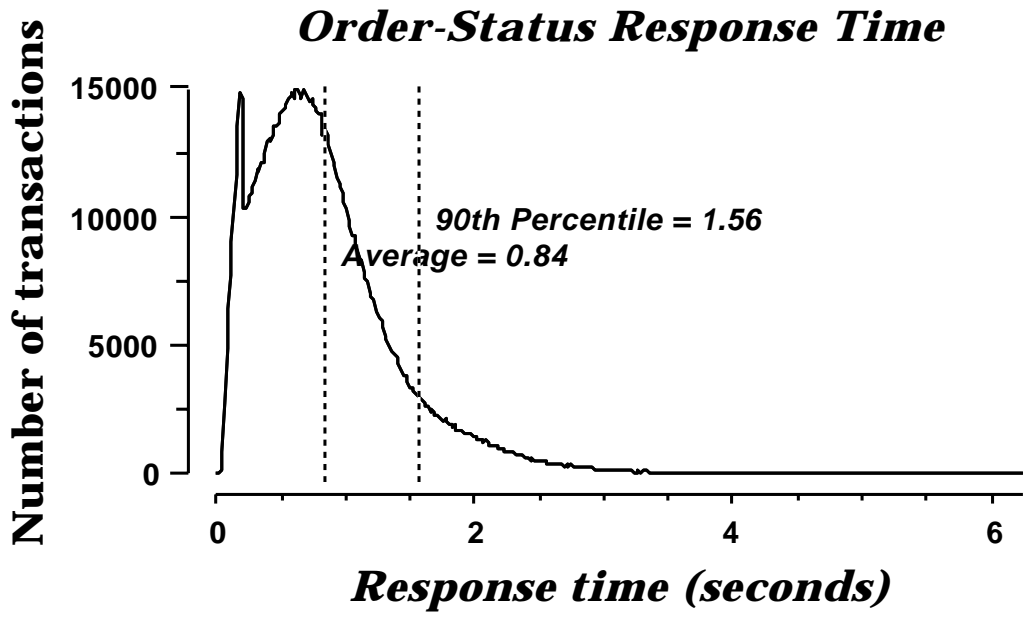
Figure 6-3-3. IBM eServer pSeries 660 Model 6M1 Order-Status Response Time Distribution
