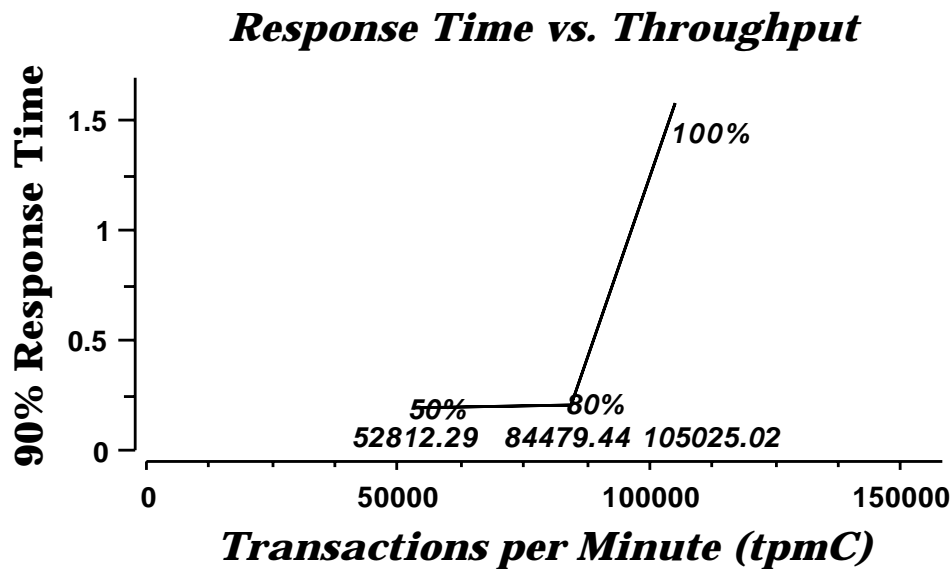
Figure 6-4-1. IBM eServer pSeries 660 Model 6M1 New-Order Response Time vs. Throughput
