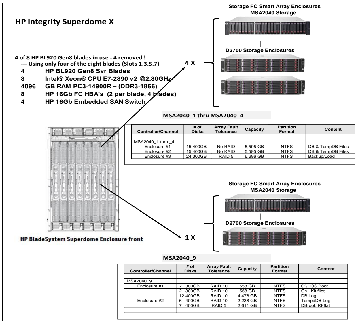
Figure 0.1 Benchmark and priced configuration for HP Integrity Superdome X
