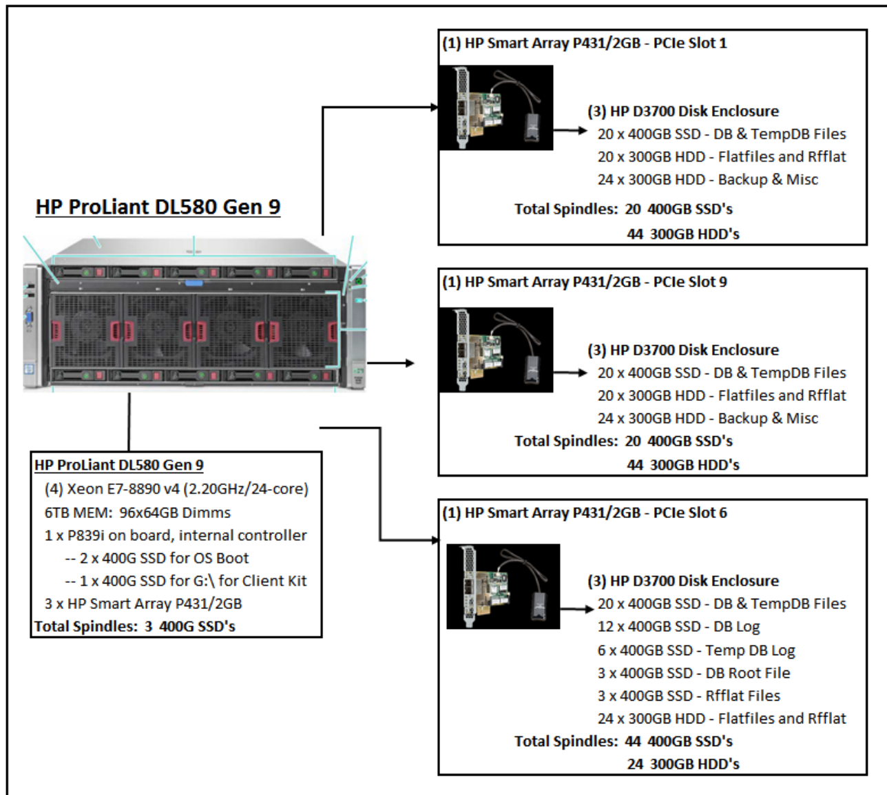
Figure 0.1 Benchmark and priced configuration for HPE ProLiant DL580 Gen9
