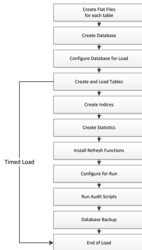
Figure 4.8: Block Diagram of Database Load Process
