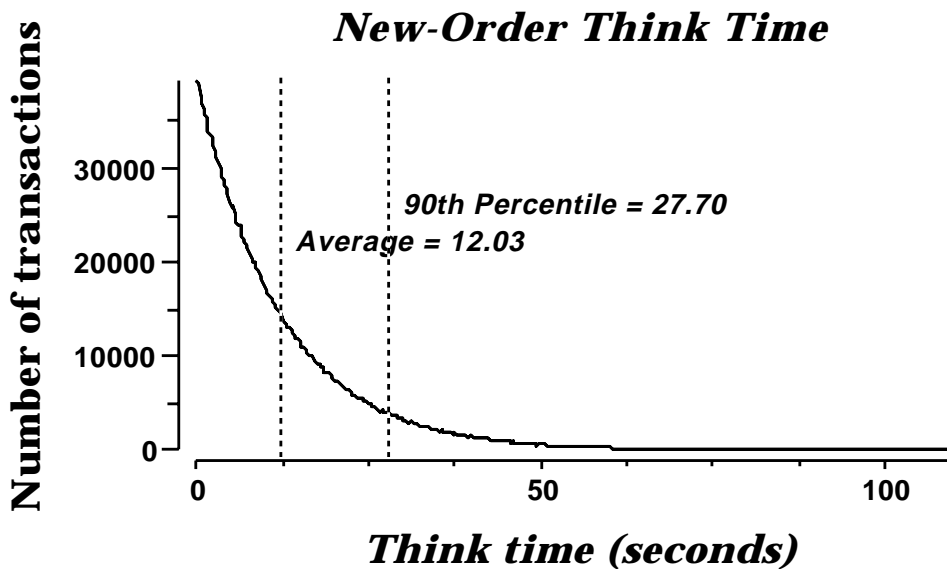
Figure 6-5-1. ESCALA EPC 810 New-Order Think Time Distribution
