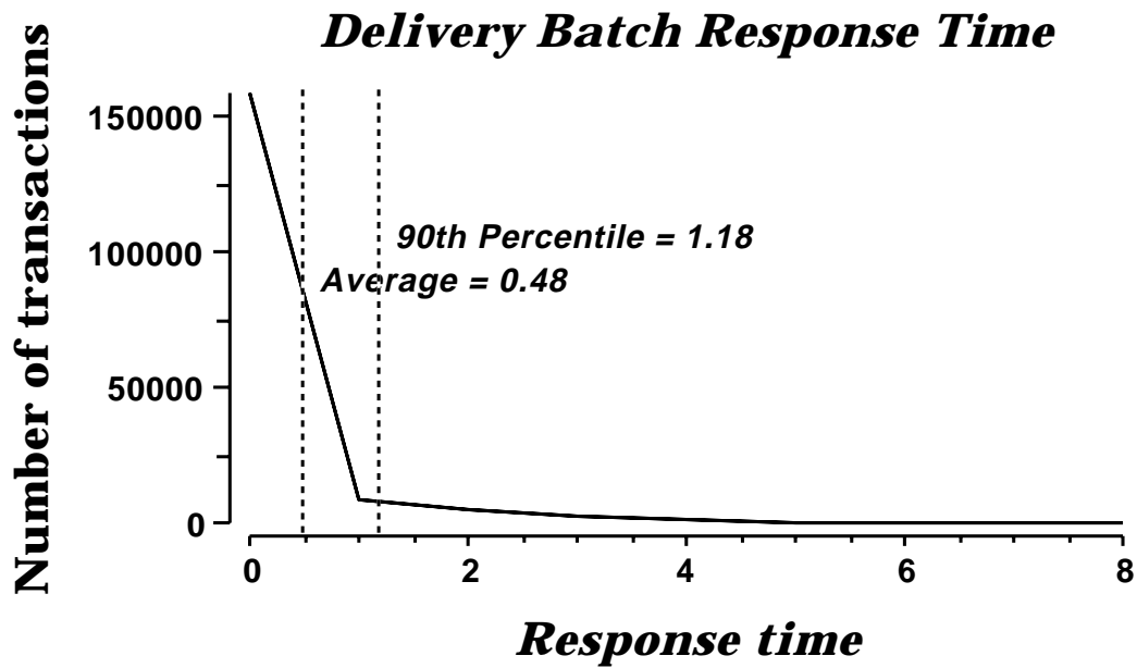
Figure 6-3-5. ESCALA EPC 810 Delivery (Deferred) Response Time Distribution
