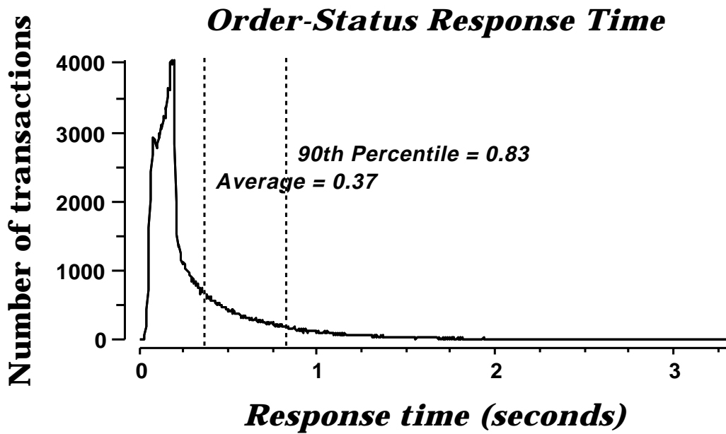
Figure 6-3-3. ESCALA EPC 810 Order-Status Response Time Distribution
