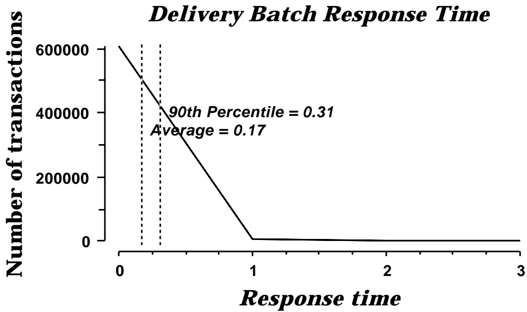
Figure 6-3-5. IBM eServer pSeries 660 Model 7026-6H1 Delivery (Deferred) Response Time Distribution
