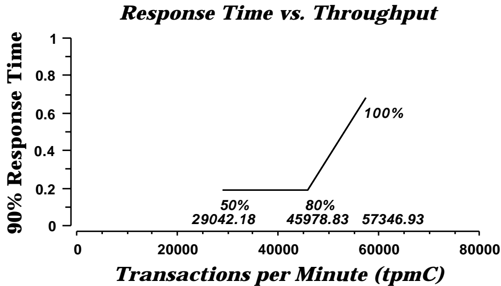
Figure 6-4-1. IBM eServer pSeries 660 Model 7026-6H1 New-Order Response Time vs. Throughput
