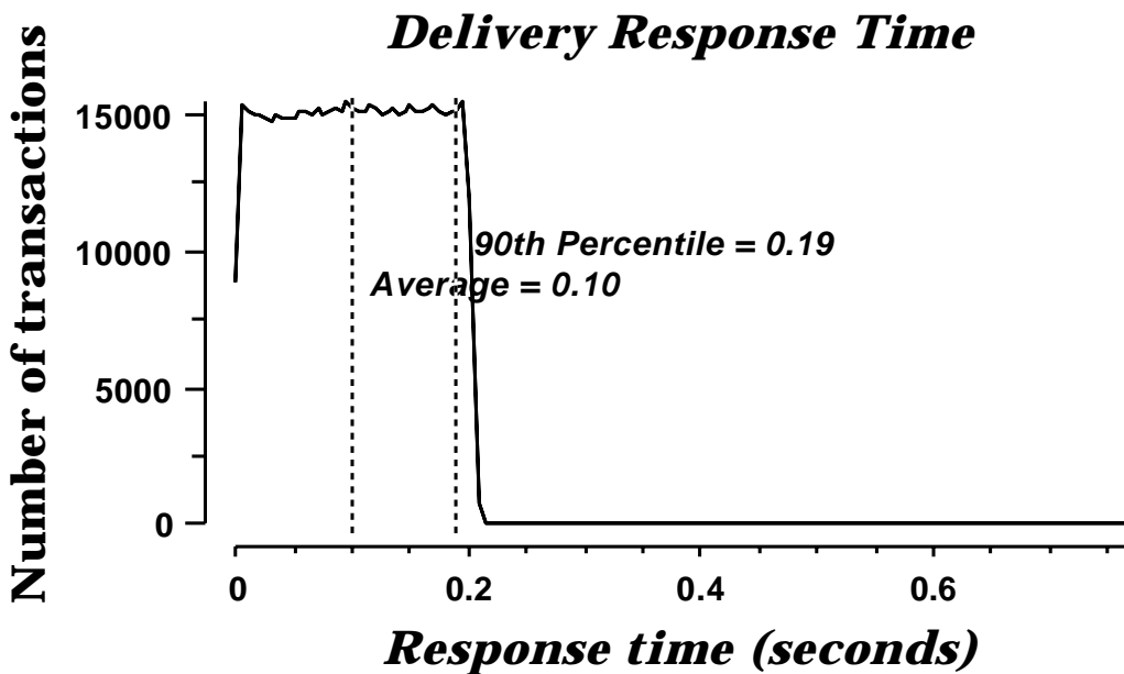
Figure 6-3-4. IBM eServer pSeries 660 Model 7026-6H1 Delivery (Interactive) Response Time Distribution
