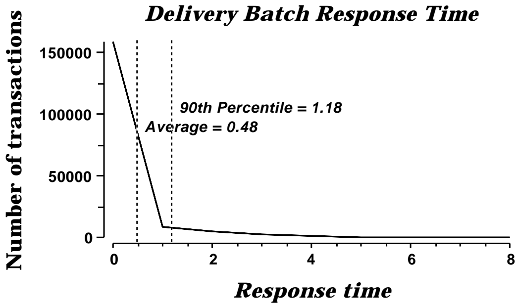
Figure 6-3-5. RS/6000 M80 Delivery (Deferred) Response Time Distribution
