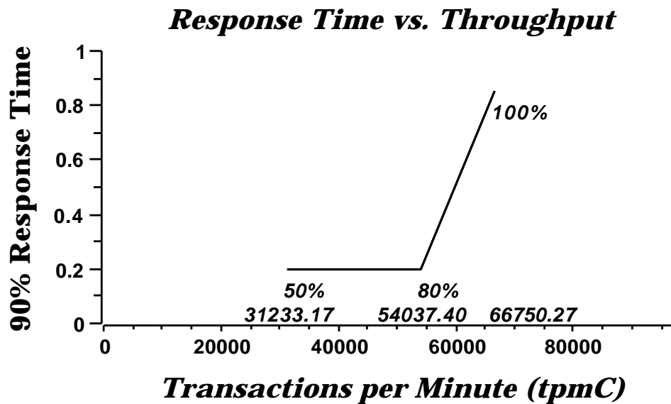
Figure 6-4-1. RS/6000 M80 New-Order Response Time vs. Throughput
