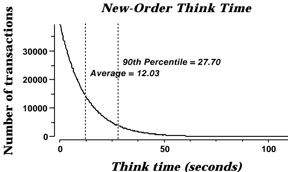
Figure 6-5-1. RS/6000 M80 New-Order Think Time Distribution
