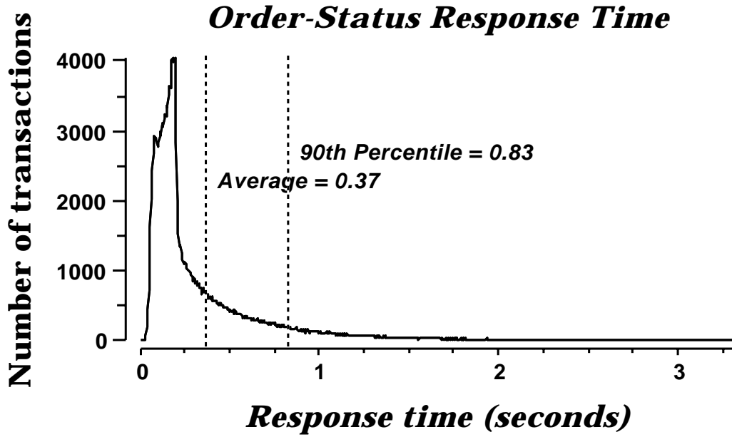
Figure 6-3-3. RS/6000 M80 Order-Status Response Time Distribution
