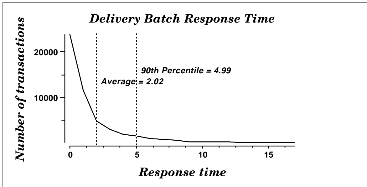
Figure 6-3-6. RS/6000 S70 Stock Level Response Time Distribution
