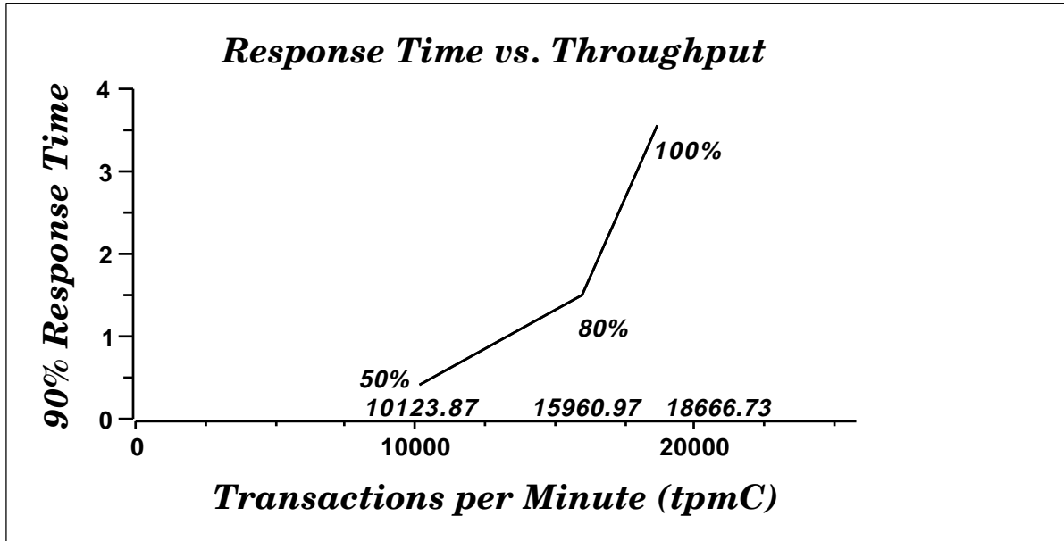
Figure 6-4-1. RS/6000 S70 New-Order Response Time vs. Throughput
