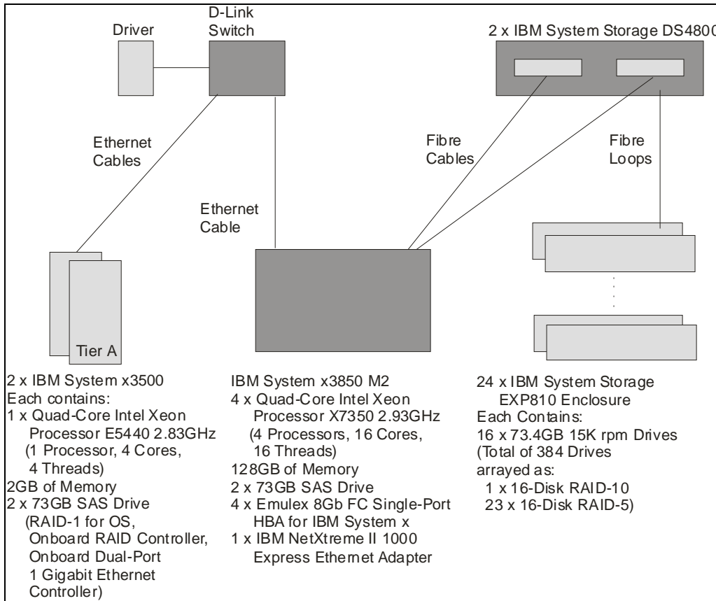
Figure 1-2. Priced Configuration
