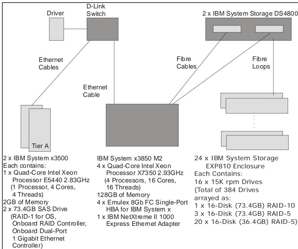
Figure 1-1. Measured Configuration
