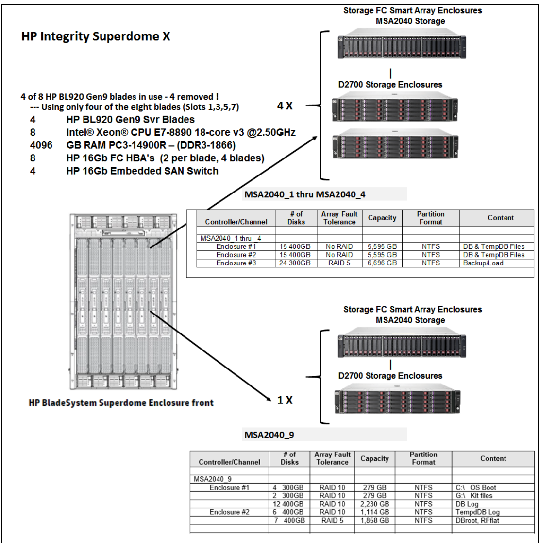
Figure 0.1 Benchmark and priced configuration for HPE Integrity Superdome X
