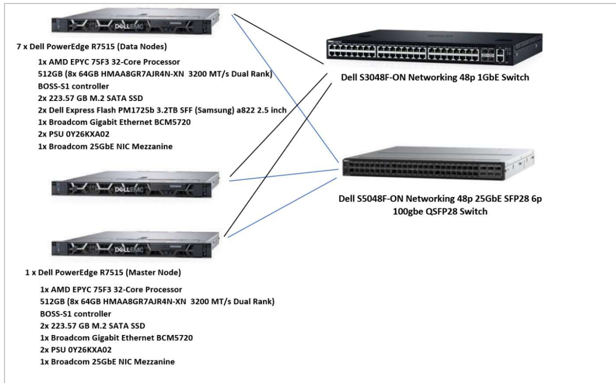
Figure 1-1 Measured Configuration
