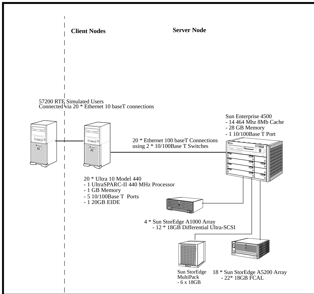
Figure 1: The Sun Enterprise 4500 Priced Configuration
